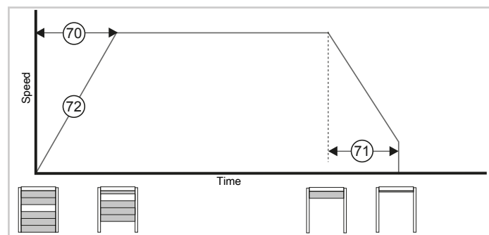
Diagram for door run and recommended settings
