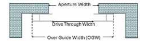
Guide Positioning
