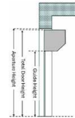
Fitting Behind the Aperture
