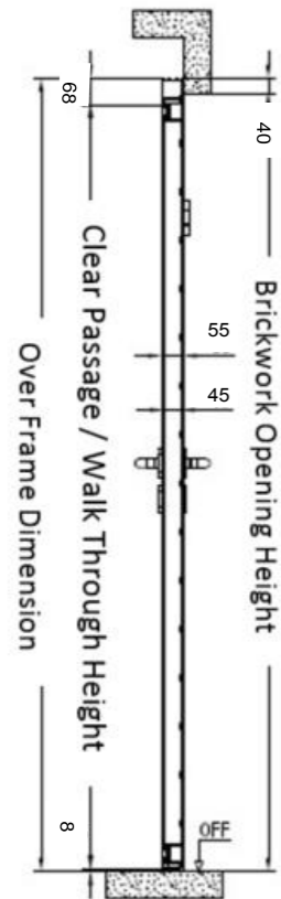
Vertical Cut (Installation behind the opening)
