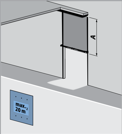
T 500 hF (B550), vertical rail system with low spring axis + steel support profile
