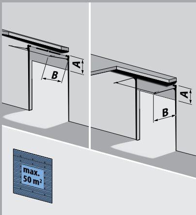
T 400 (B350), elevated rail system
