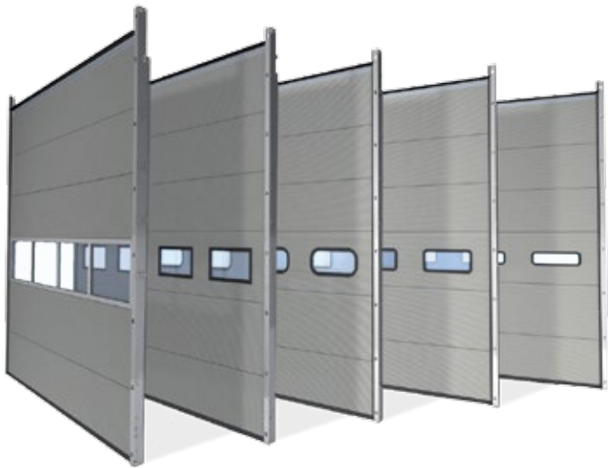
U-value Thermo 40 mm sectional door: 5,000 x 5,000 mm: 1.02 W/m 2 K
