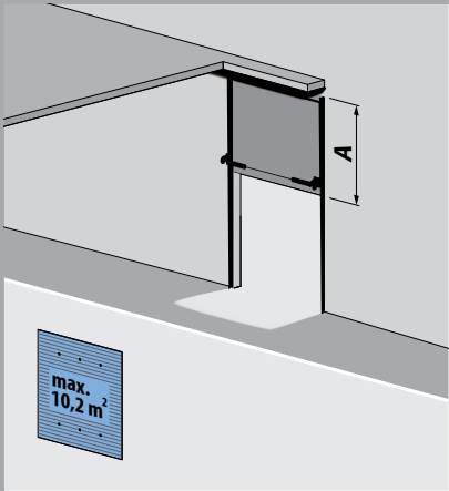
T 500 DS (B550 dock), vertical rail system with low spring axis
