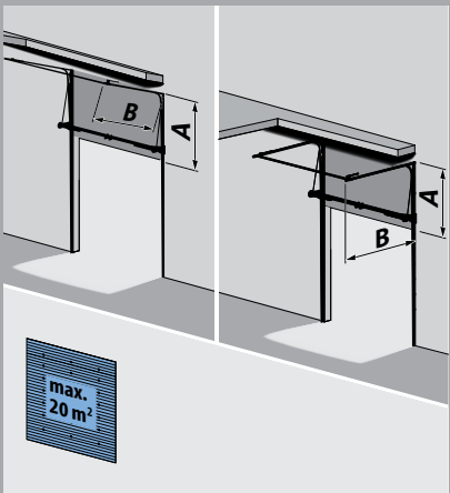
T 400 hF (B350), elevated rail system with low spring axis + steel support profile
