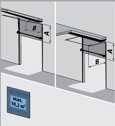
T 400 DS (B350 dock), elevated rail system with low spring axis
