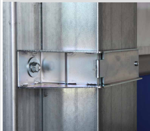
Integrated curtain stiffener/hinge profiles
