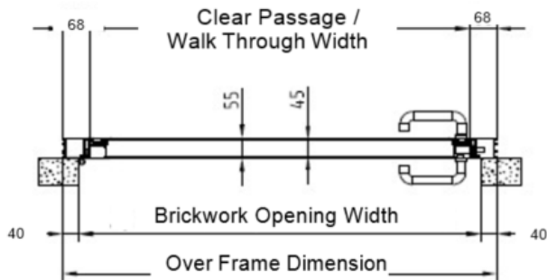
Horizontal Cut (Installation behind the opening)
