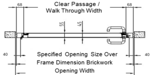
Horizontal Cut (Installation behind the opening)
