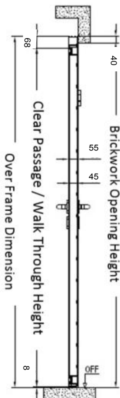
Vertical Cut (Installation behind the opening)
