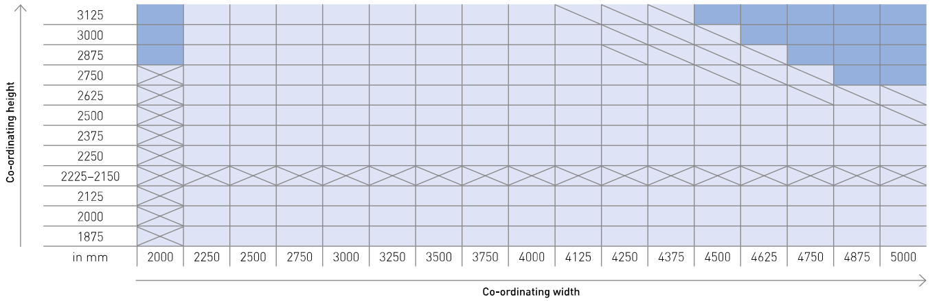
Size range for Sectional doors with pass door
