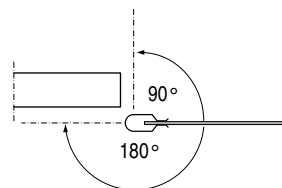
Arrangement 2 1 x 90° and 1 x 180° in front of the clear opening
